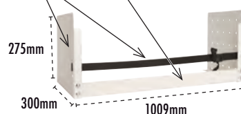
Floor Mount Enclosure with Removable Front Angle & Strap. Ideal for large buckets
