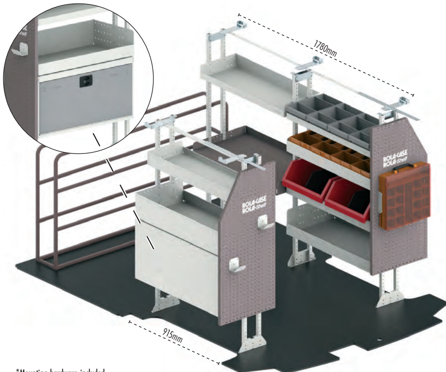
Full Shelving Package #RSSWBSV
